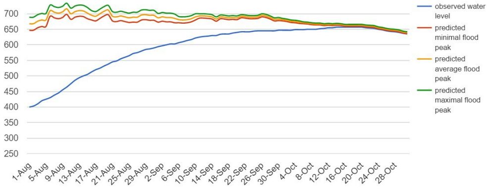
Water level measurements and predictions of the flood peak in Mopti
